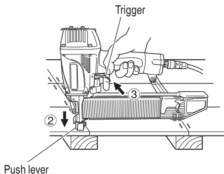
(2) Continuous operation (Push lever fire)
